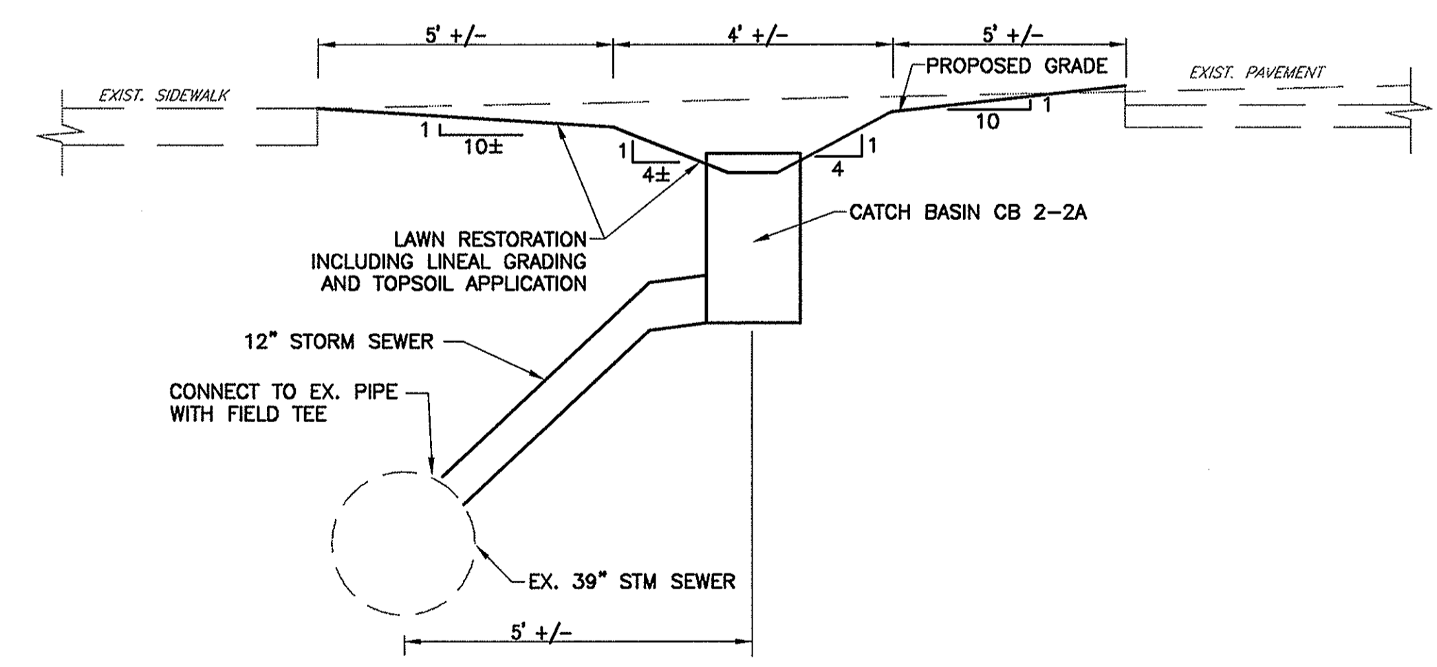
SECTION A-A NO SCALE
