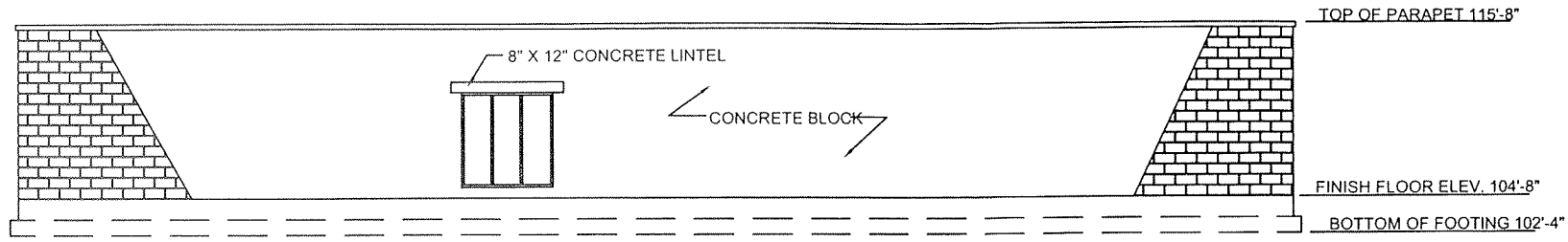
1 SOUTH ELEVATION SCALE:
