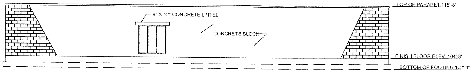
1 SOUTH ELEVATION SCALE:
