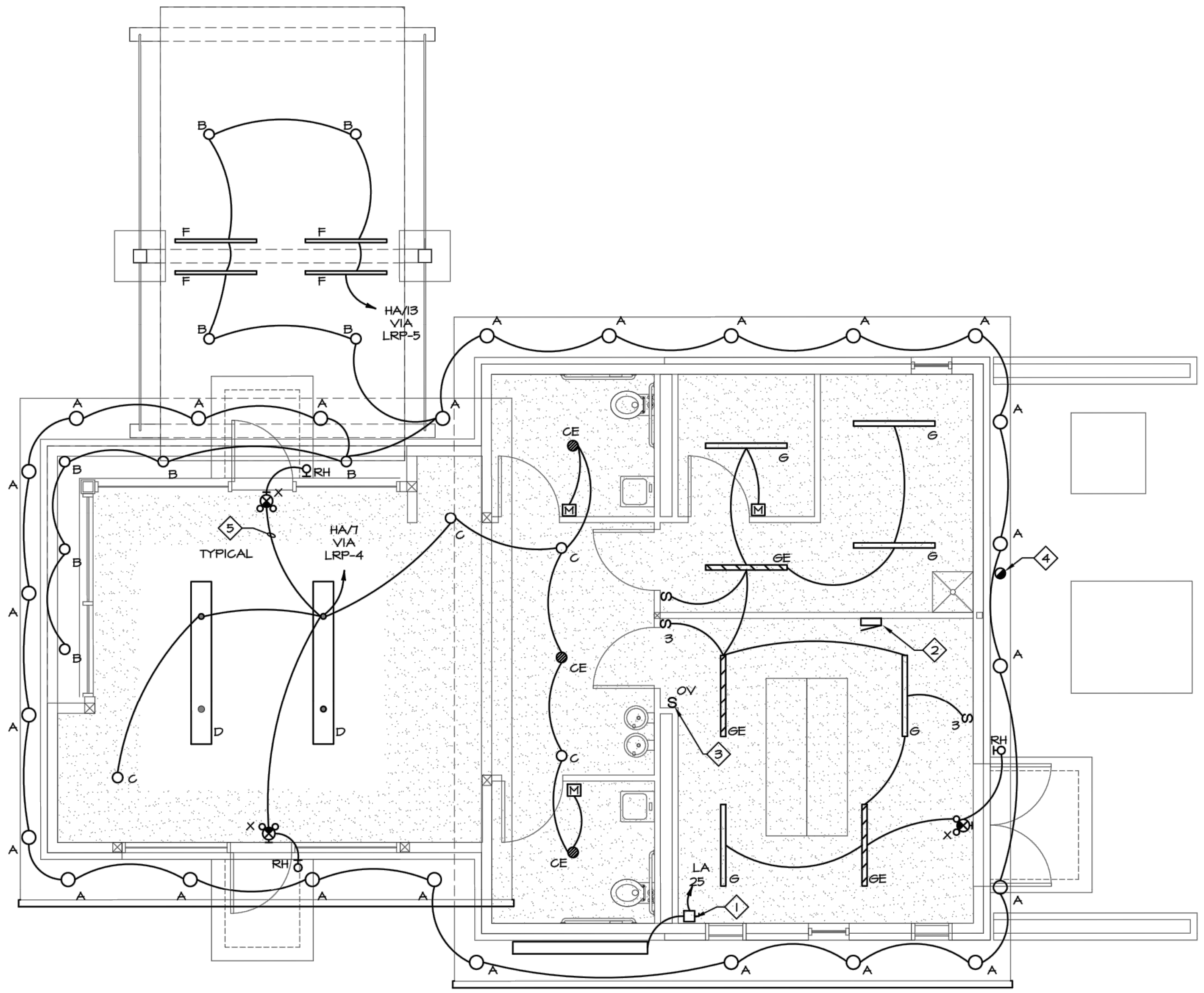
LIGHTING PLAN SCALE: 1/4" = 1'-0"
