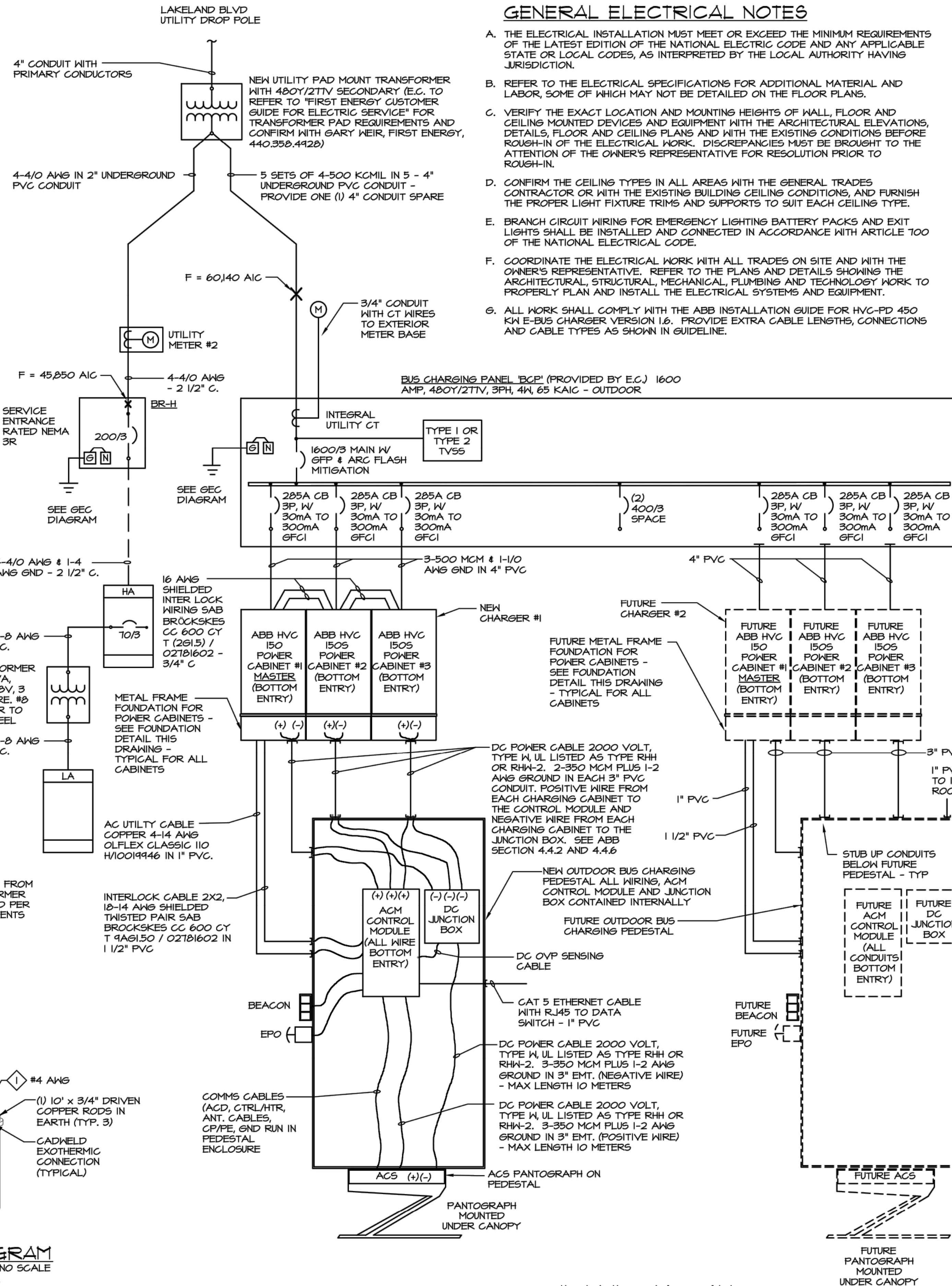
ONE LINE DIAGRAM NO SCALE
