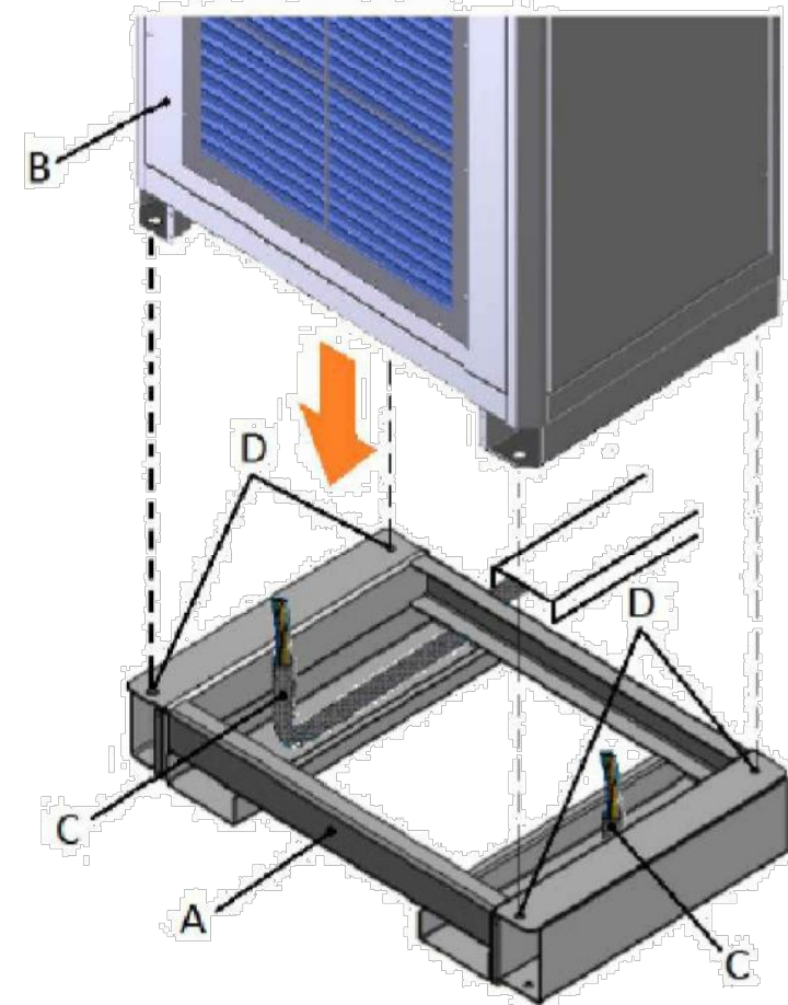
PART A - FOUNDATION PART B - POWER CABINET PART C - CABLES PART D - TAPPED HOLES
