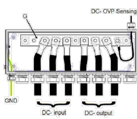
JUNCTION BOX INSTALLATION SHALL COMPLY WITH ABB INSTALLATION SPEC SECTION 5.16.4
