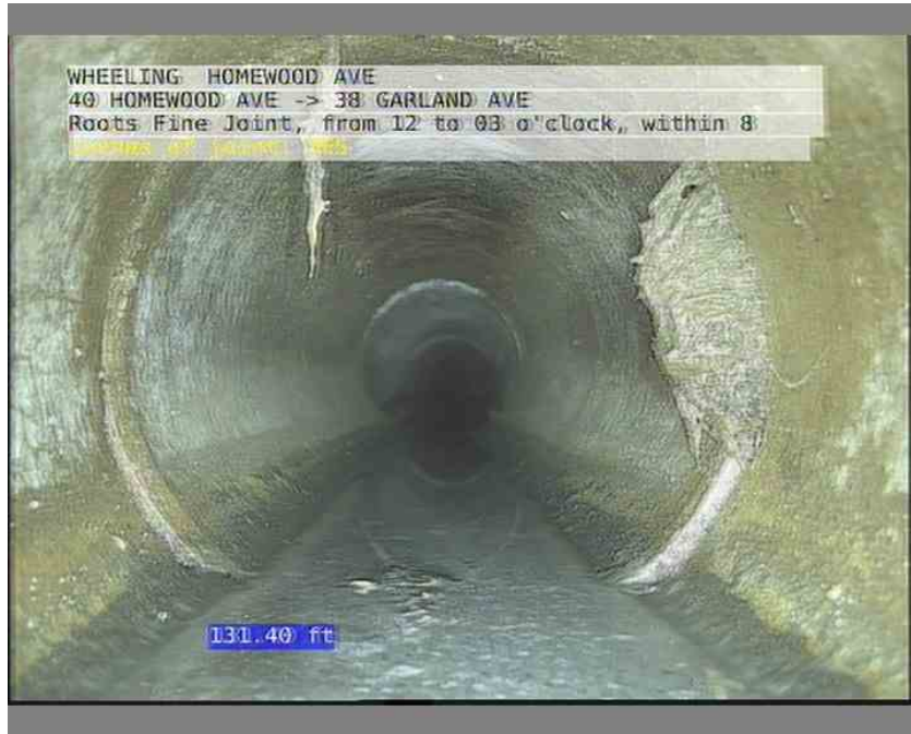
11, 00:10:37, 131.40ft Roots Fine Joint, from 12 to 03 o'clock, within 8 inches of joint: YES
