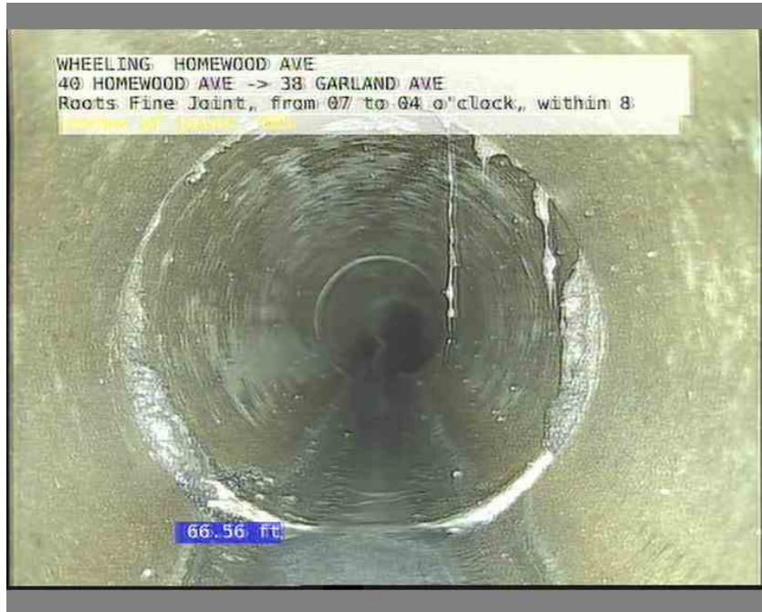
7, 00:06:29, 66.56ft Roots Fine Joint, from 07 to 04 o'clock, within 8 inches of joint: YES
