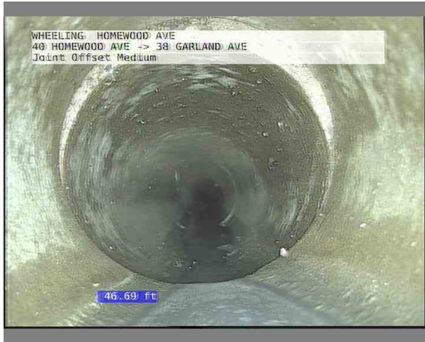
5, 00:05:12, 46.69ft Joint Offset Medium
