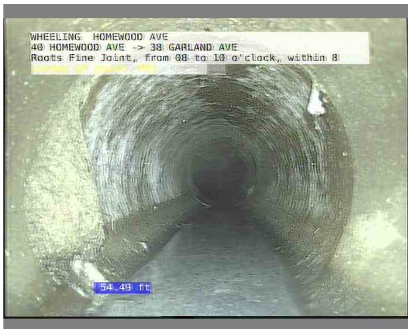
6, 00:05:45, 54.49ft Roots Fine Joint, from 08 to 10 o'clock, within 8 inches of joint: YES
