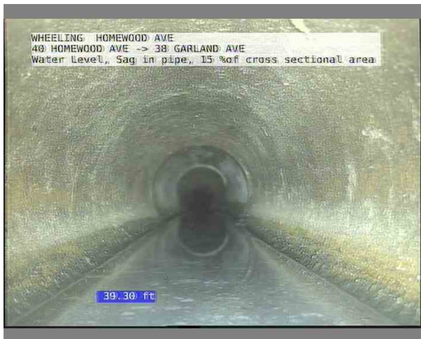
4, 00:04:30, 39.30ft Water Level, Sag in pipe, 15 %of cross sectional area
