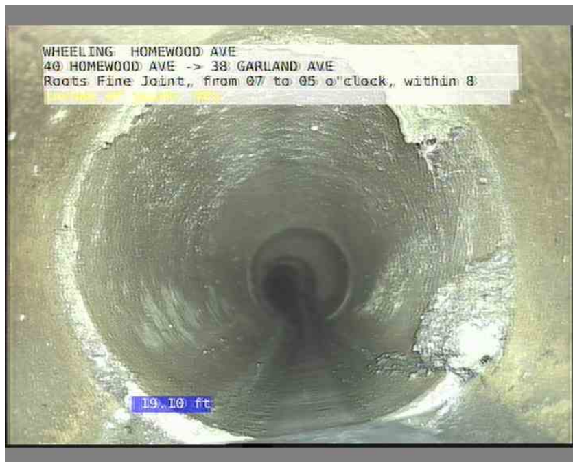
2, 00:03:15, 19.10ft Roots Fine Joint, from 07 to 05 o'clock, within 8 inches of joint: YES
