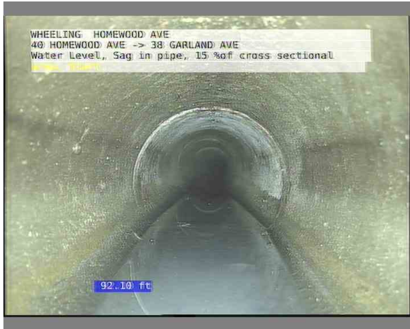
9, 00:08:05, 92.10ft Water Level, Sag in pipe, 15 %of cross sectional area, Start
