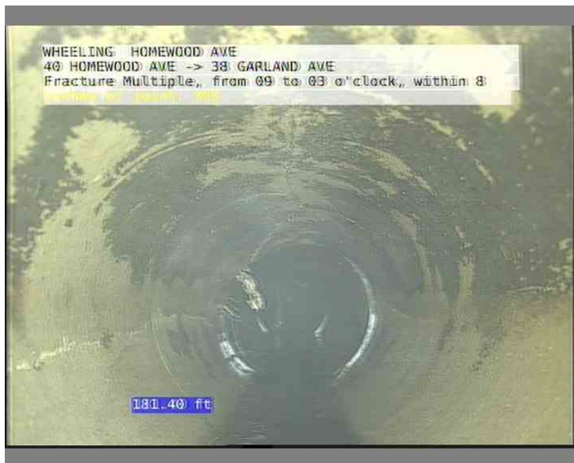
14, 00:15:04, 181.40ft Fracture Multiple, from 09 to 03 o'clock, within 8 inches of joint: YES
