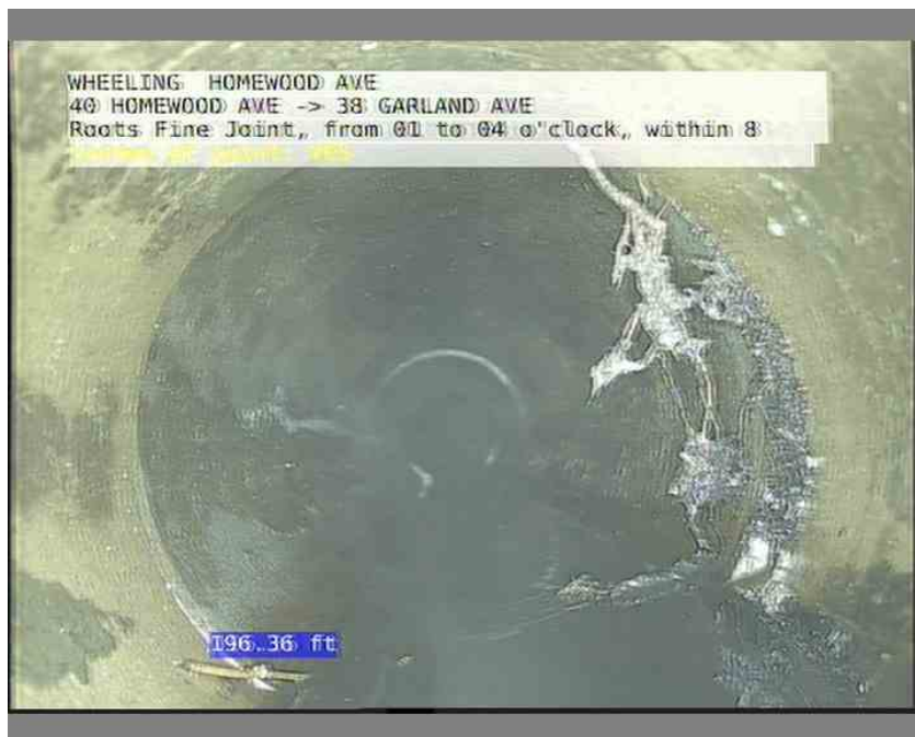
16, 00:16:36, 196.36ft Roots Fine Joint, from 01 to 04 o'clock, within 8 inches of joint: YES
