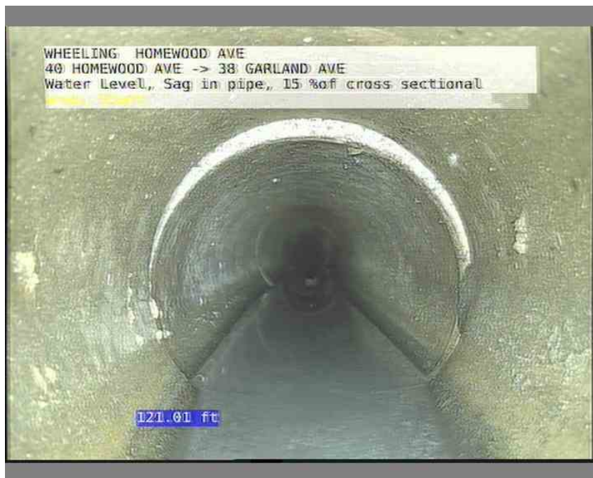
10, 00:09:47, 121.01ft Water Level, Sag in pipe, 15 %of cross sectional area, Start
