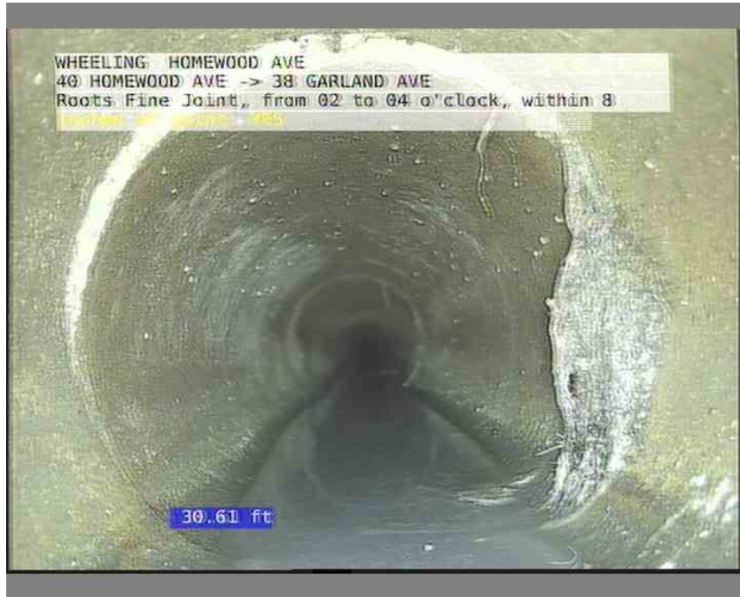
3, 00:03:57, 30.61ft Roots Fine Joint, from 02 to 04 o'clock, within 8 inches of joint: YES
