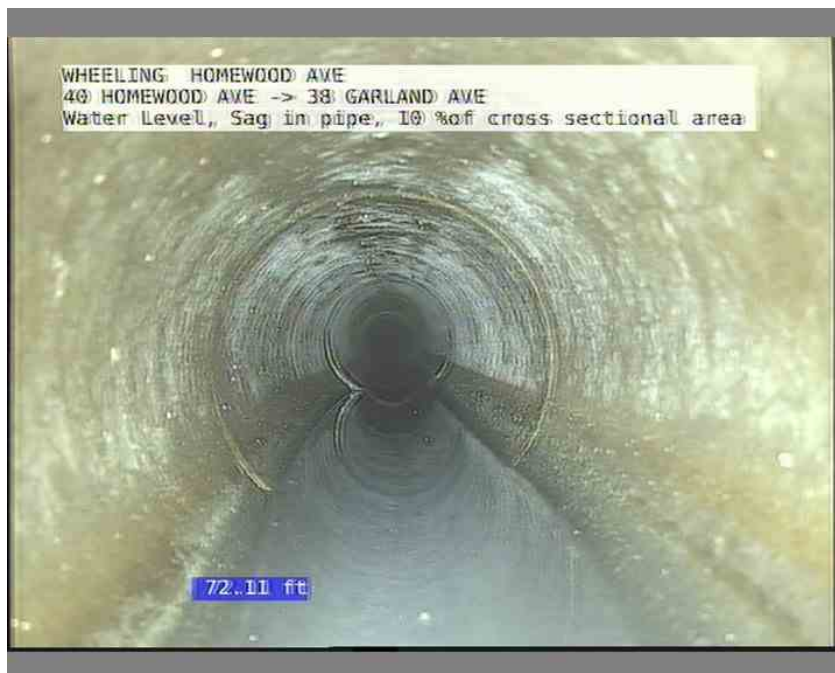
8, 00:07:01, 72.11ft Water Level, Sag in pipe, 10 %of cross sectional area, Start
